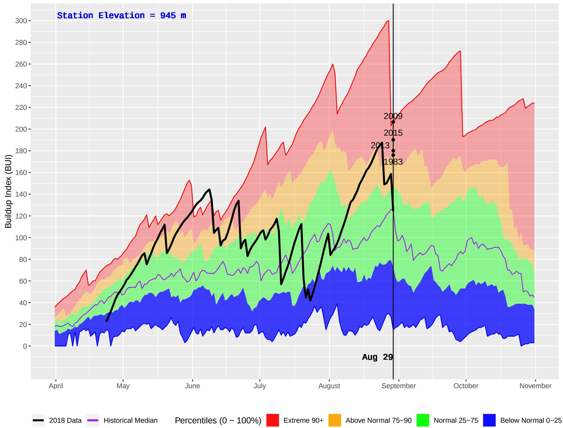
TATLA LAKE HUB (208) : Historical (1980–2016) and Current (2018) Daily Buildup Index (BUI)
